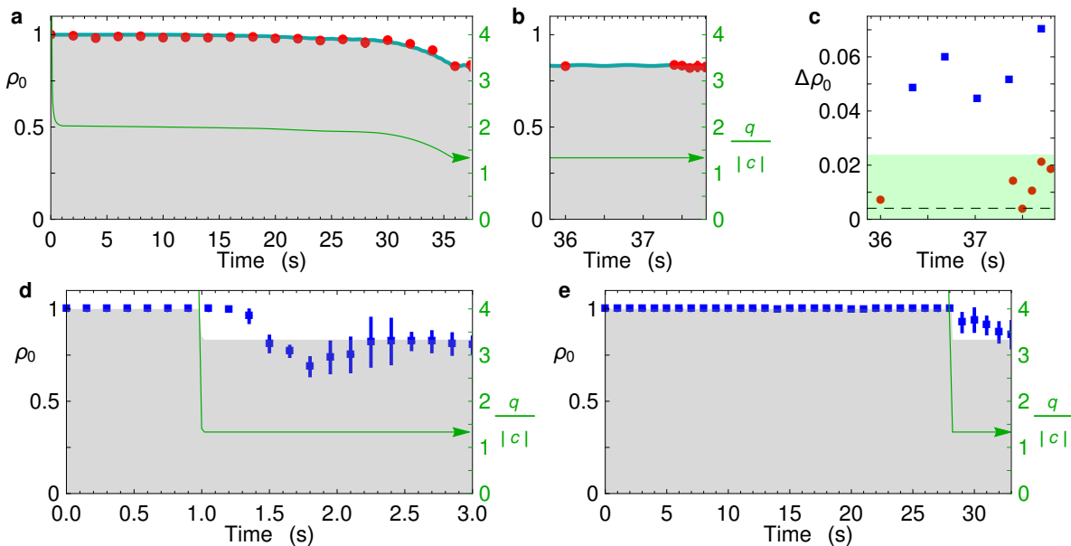
FIG. 3. Adiabatic and nonadiabatic dynamics. a-c , Adiabatic dynamics of population \rho_0 and the uncertainty \Delta\rho_0 (see texts). d-e , Non-adiabatic dynamics of population \rho_0 of 1 s and 28 s linear ramp from q/|c| = 140 \rightarrow 1.33 . Red circle (blue square) markers are the adiabatic (nonadiabatic) measurements, gray shaded regions are the theoretical \rho_{0,GS} values, green arrow lines represent the ramp of q/|c| (vertical axis on the right), and cyan curves represent the dynamics simulation of \rho_0 with the corresponding q/|c| ramp. Each adiabatic data point is an average of 3 measurements and each non-adiabatic data point is an average of 15 measurements. ( Color online ).
